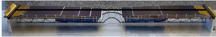
Figure 4.25: Image showing the central ladder with the shift in the perforated tube.
