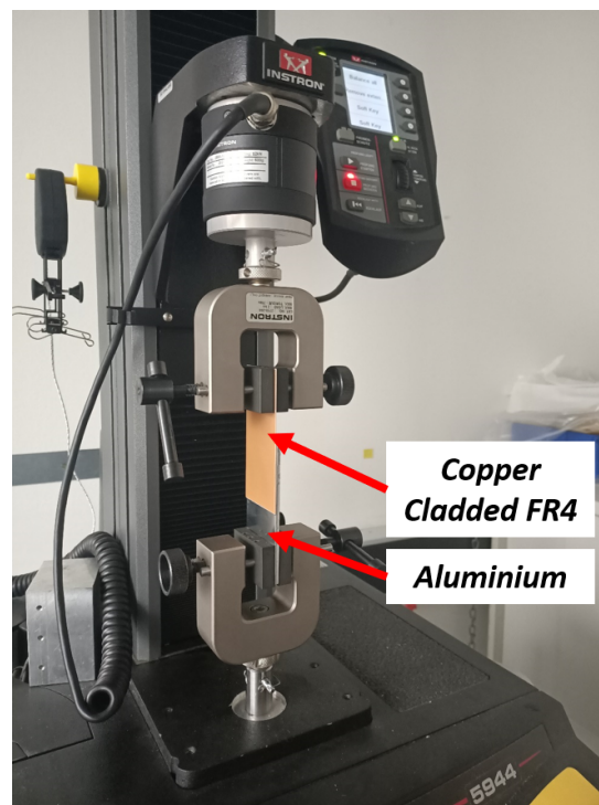
Figure 2.9: Front-view of Instron 5940 testing machine to perform the lap shear test. At the bottom grip, the aluminum sheet is clamped and the copper sheet is fixed on the top grip which is pulled at 180° until the surfaces are separated or maximum limit of the software is reached.
