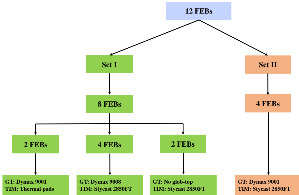
Figure 2.44: Flow chart showing the division of the FEBS into two sets of measurements, where GT refers to Glob-top material and TIM refers to the Thermal Interface material.
