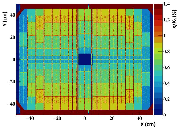
Figure 3.1: Material budget simulation for station 7 (last station) of STS.
