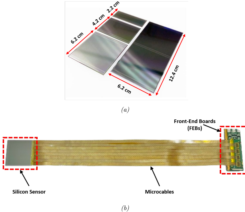
Figure 1.8: (a) Variants of Silicon sensors with width of sensor equals 6.2 cm and length varies from 2.2 cm, 4.2 cm, 6.2 cm and 12.4 cm distributed over the stations. (b) STS module after connecting to its components. The module afterwards is covered with the shielding layer and the FEBs are glued to the cooling shelves.
